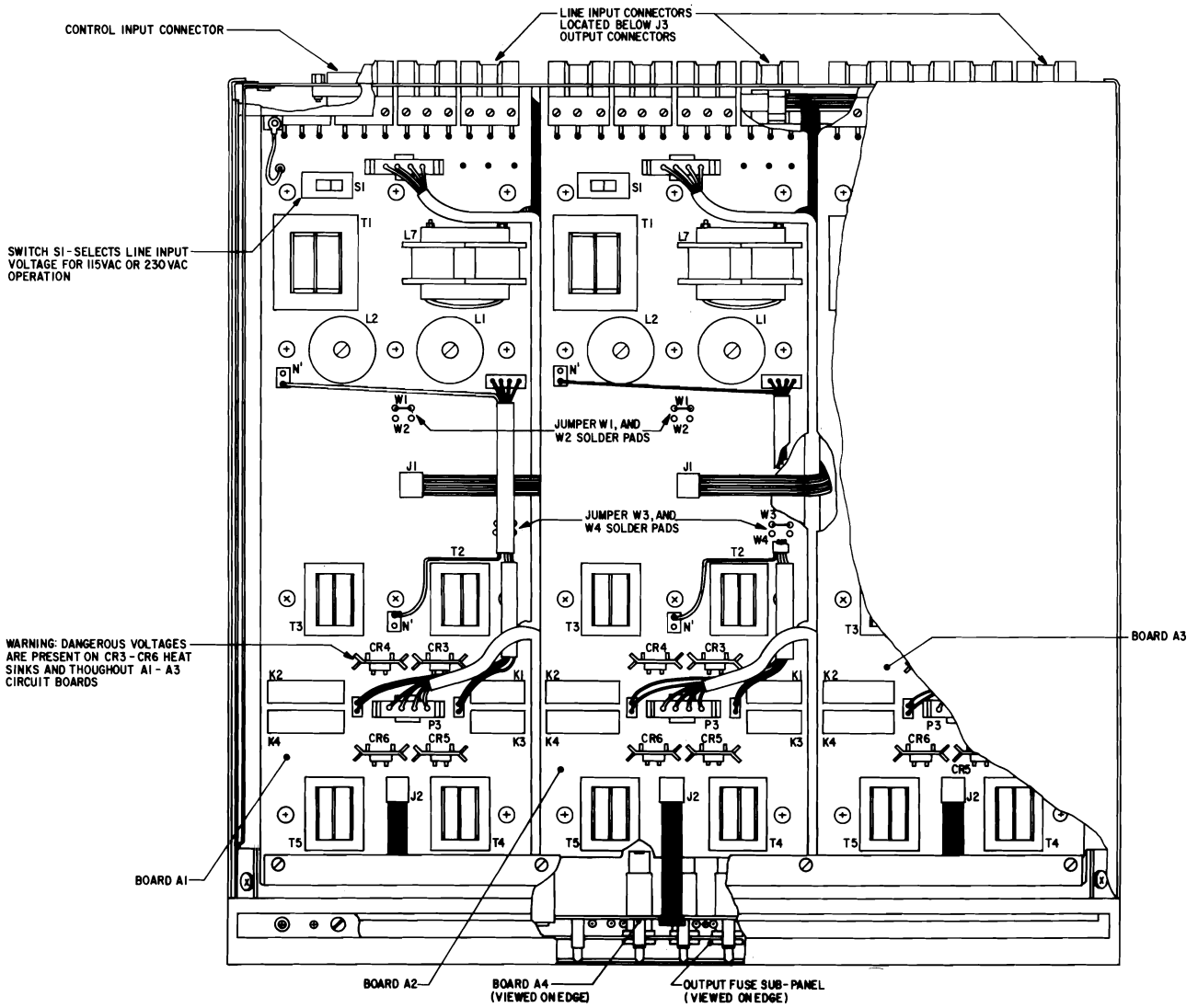
Figure 7-2A. Assembly Locations.
