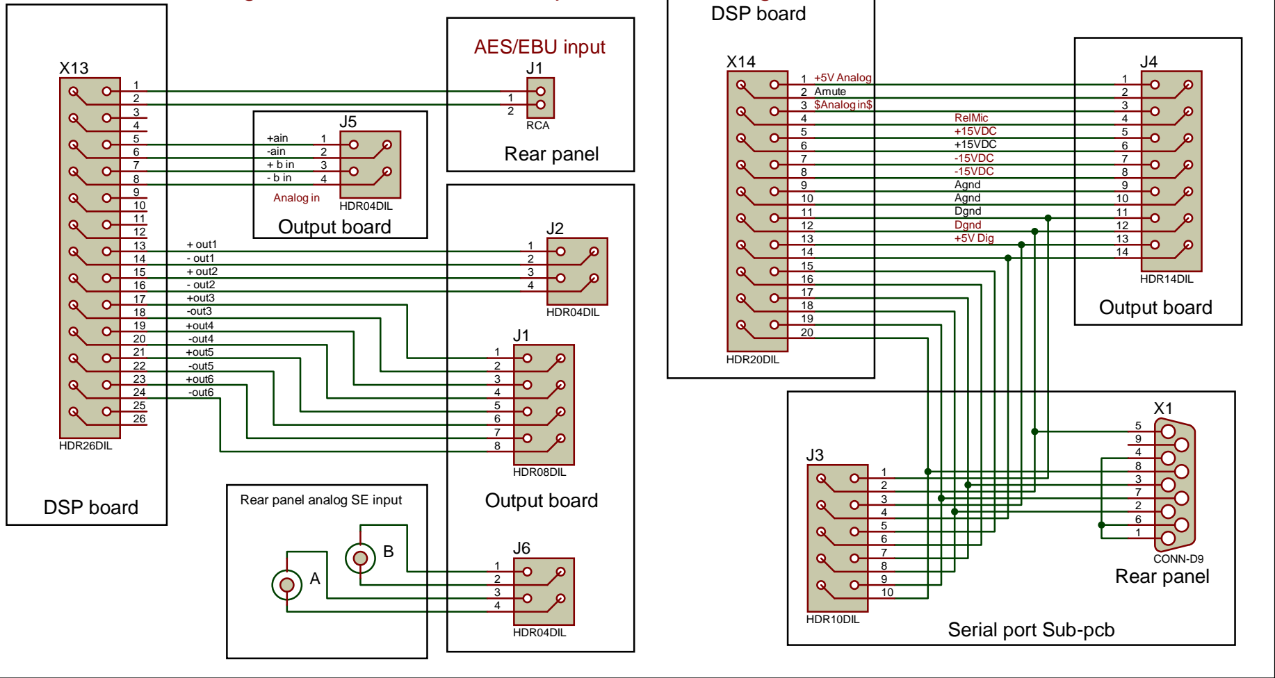
Fig 6 B DCX2496 Active output flatcable wiring
