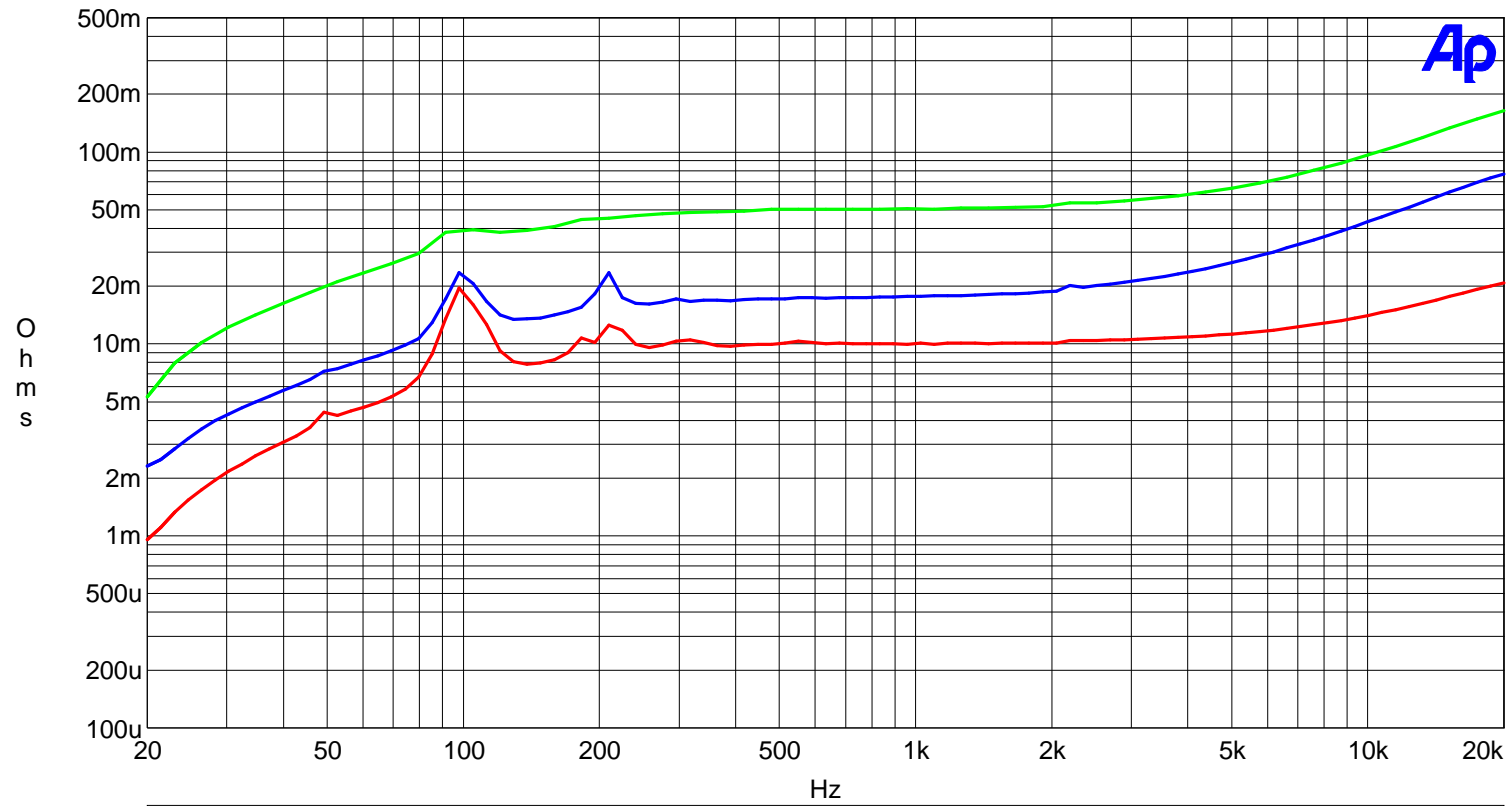
Fig 3 - T-reg output impedance versus frequency
